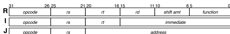
(b) MIPS basic instruction formats
